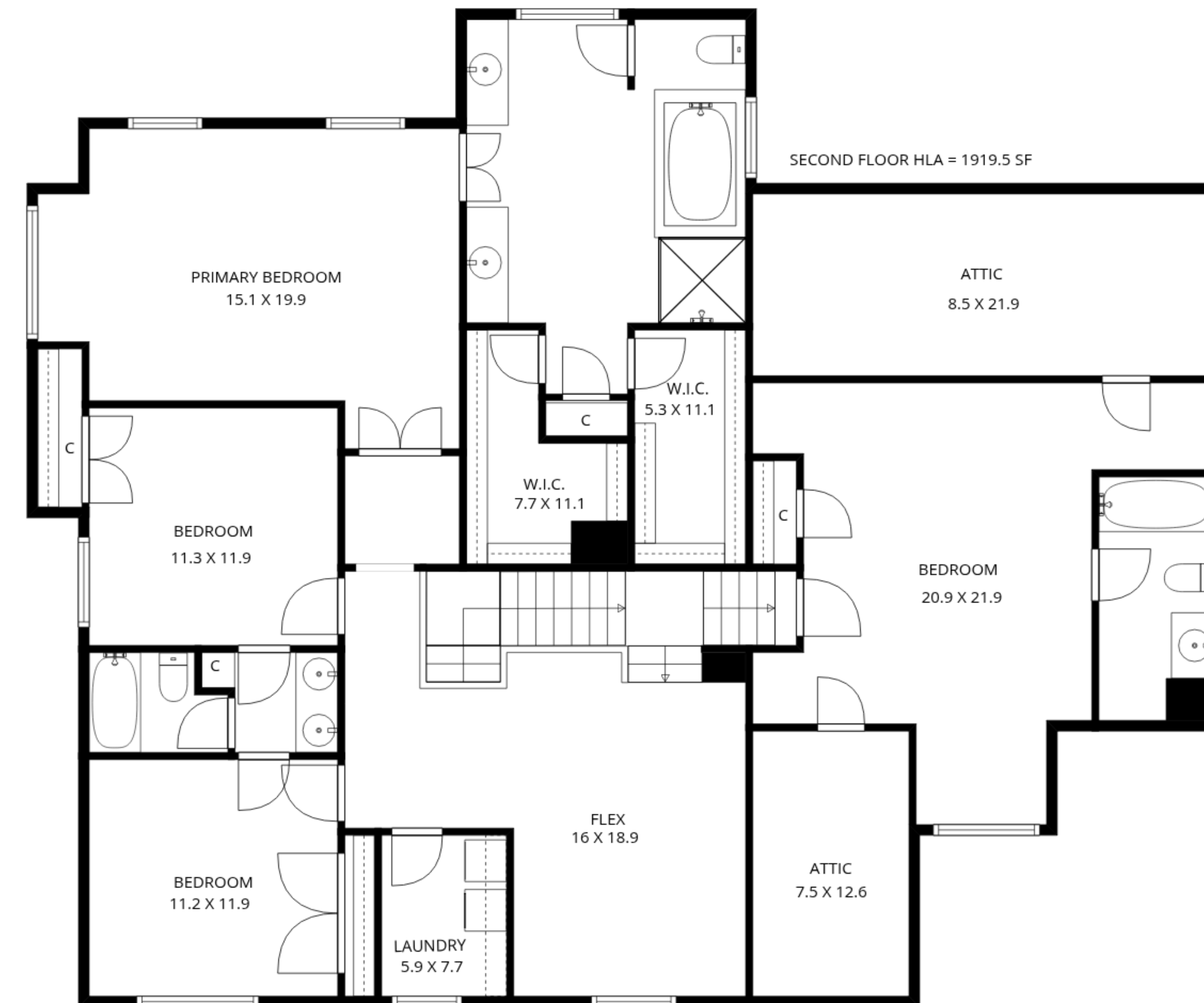
3rd floor
